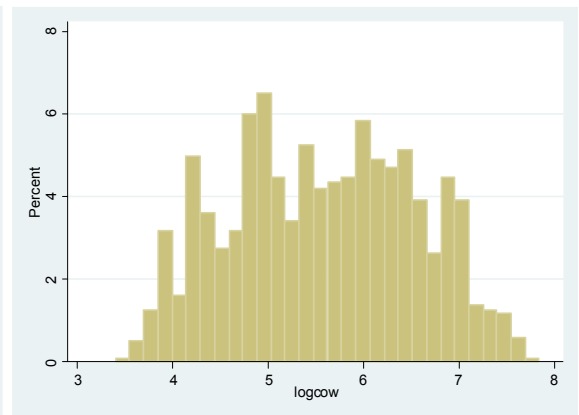
Figure 4. Dist. of logcow
