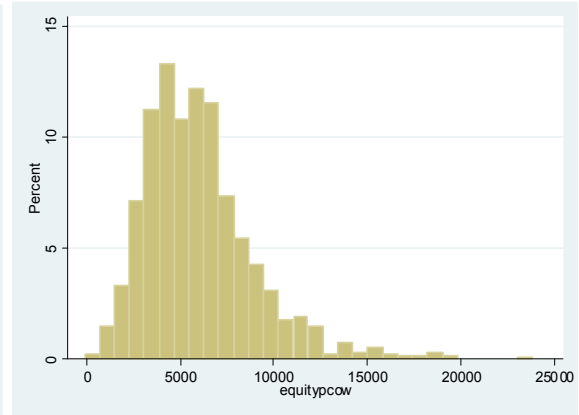
Figure 2. Dist. of equitypcow
